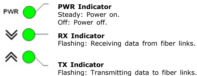
FIGURE 4: LED INDICATIONS
