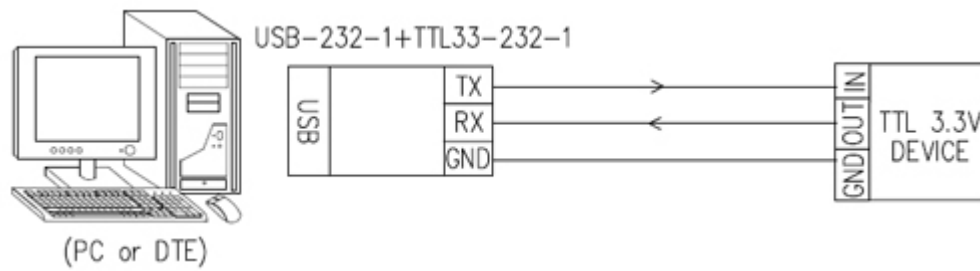
(FIGURE 1: USB-TTL 3.3V CONVERTER CONNECTION DIAGRAM)
